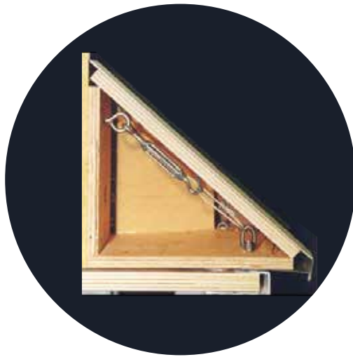
Hanging System used in conjunction with Wood Roof System
